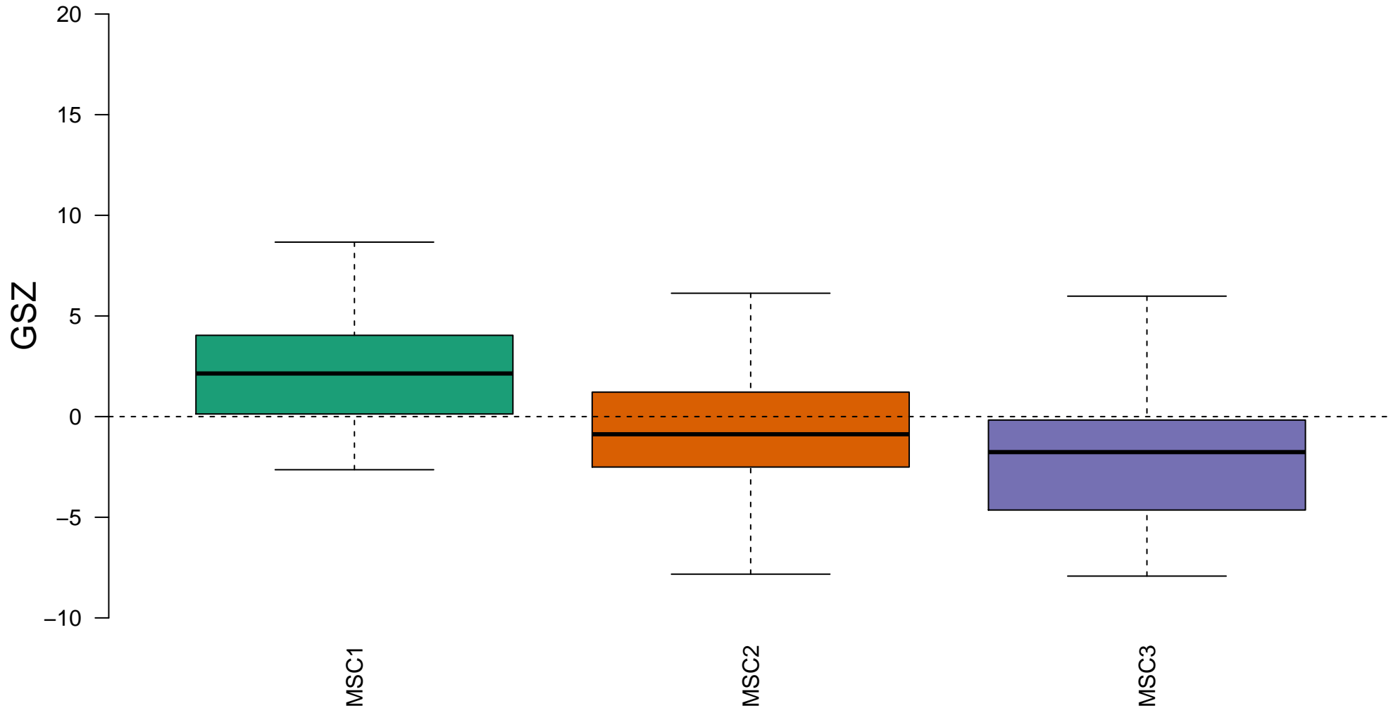
Overlap_fetal_midbrain_ReprPC
